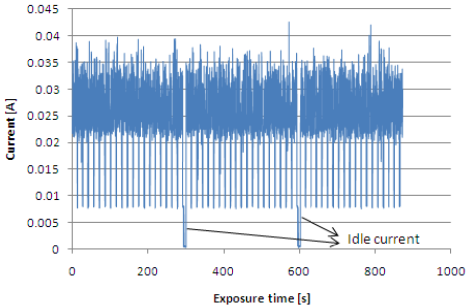
Figure 8: Supply current during gamma exposure.
