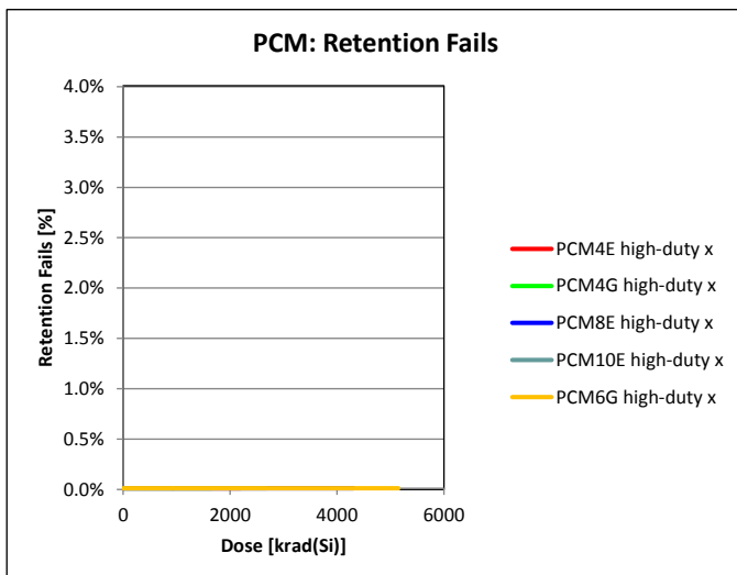
Figure 7: Retention errors versus dose during x-ray irradiations.
