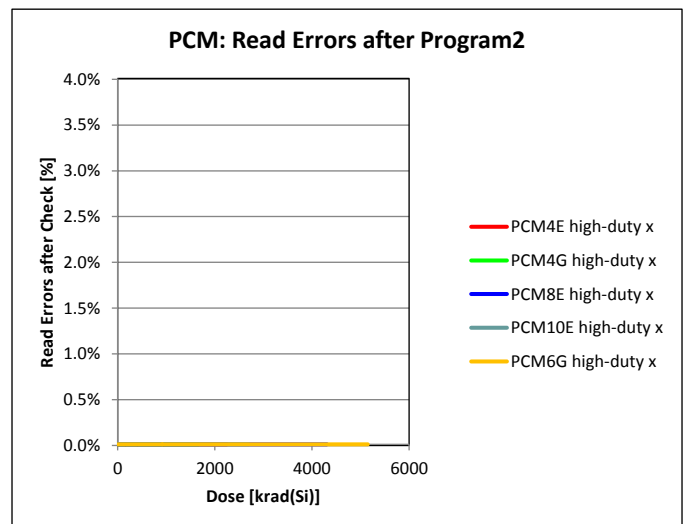
Figure 6: Read fails after Program2 versus dose during x-ray irradiations.
